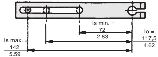
Fig. 23: Balancín
